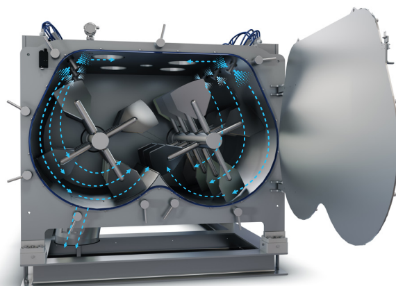
The air jets spread along the surfaces, blowing particles in the air which are then vacuumed through the outlet.
