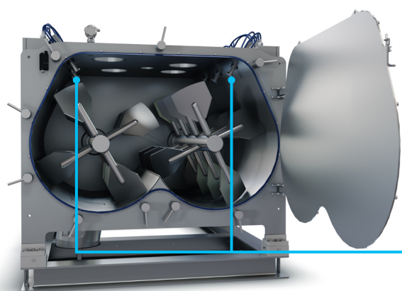
Pop-up nozzles are located on the top corners of the mixer's ceiling.
