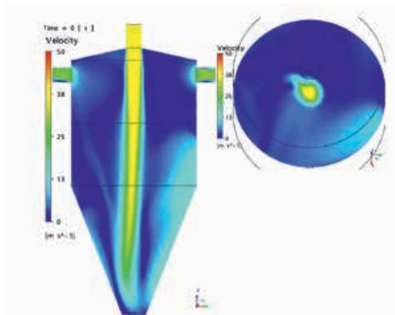
Case: simulated air velocity profile inside the drying chamber
